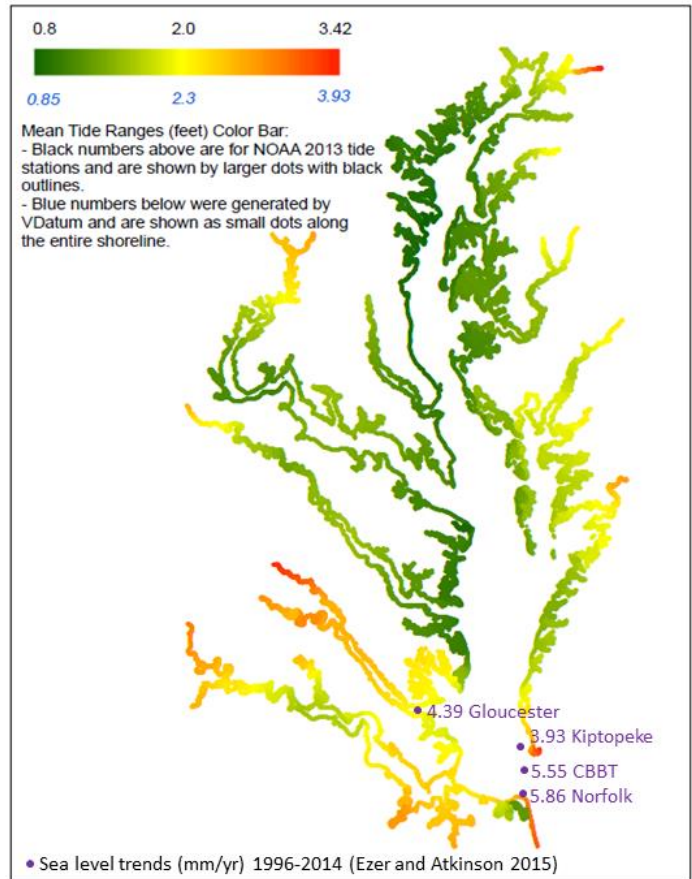
Figure 3. Tide range and sea level trends around the Bay
