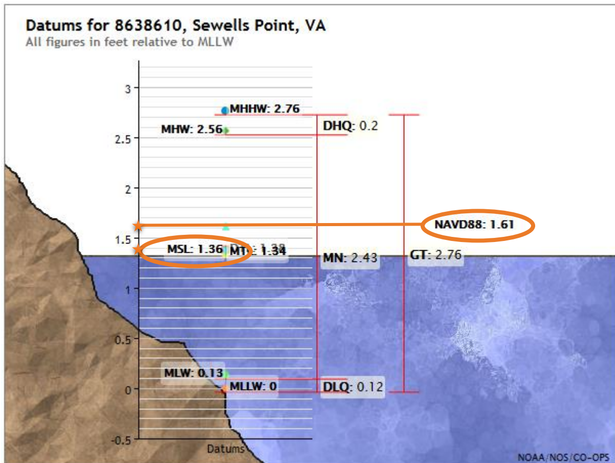
Figure 4. Tidal datum chart for Sewell's Point. All data relative to MLLW in the current tidal datum. Source: https://tidesandcurrents.noaa.gov/datums.html?id=8638610
