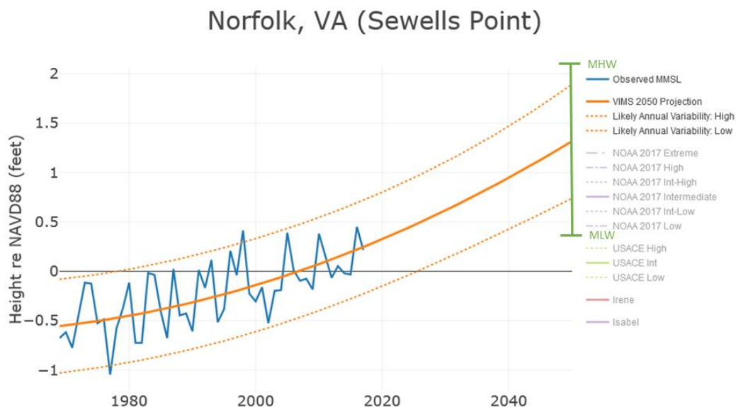
Figure 2. Tide range above 2050 projection
